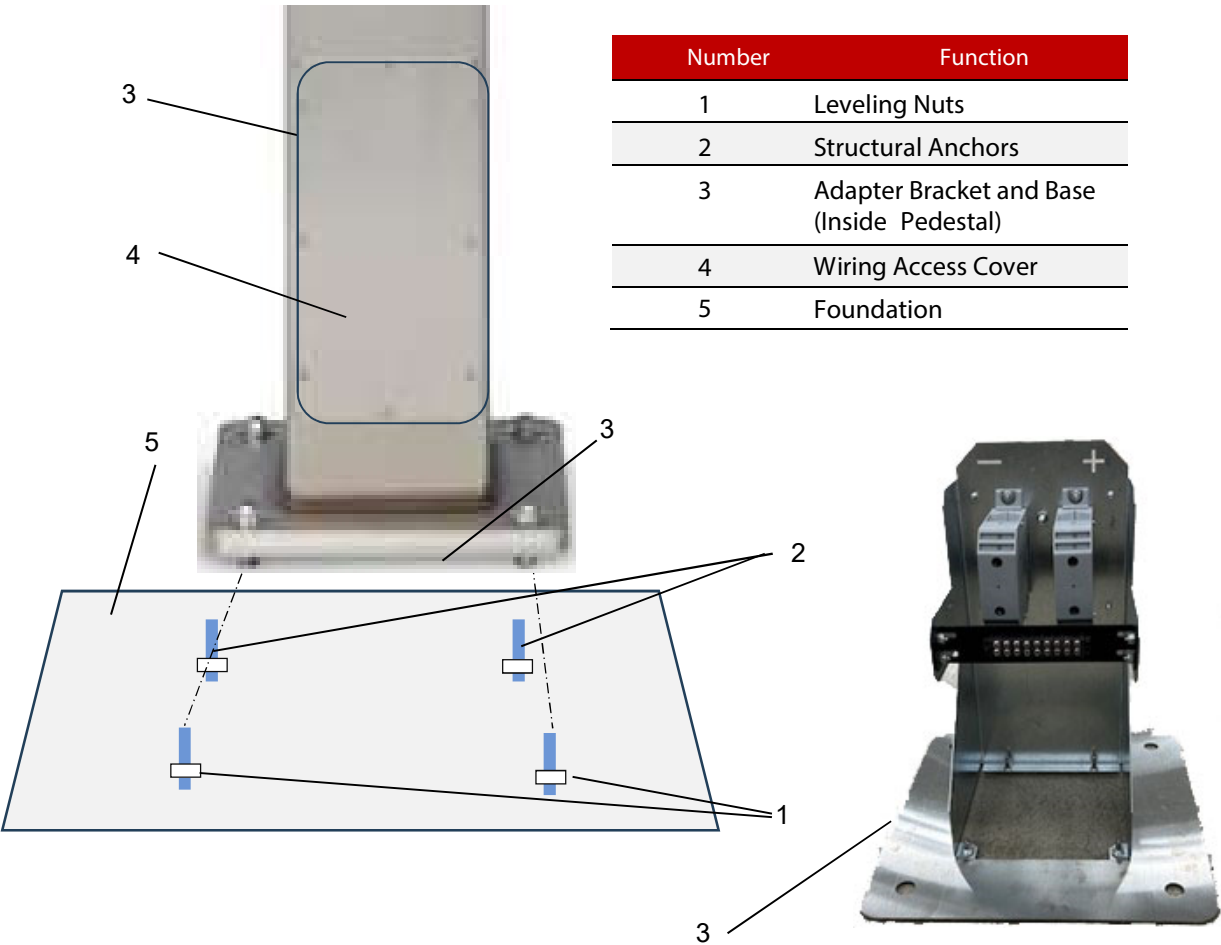
Figure 19 Pedestal, Adapter Bracket and Base
